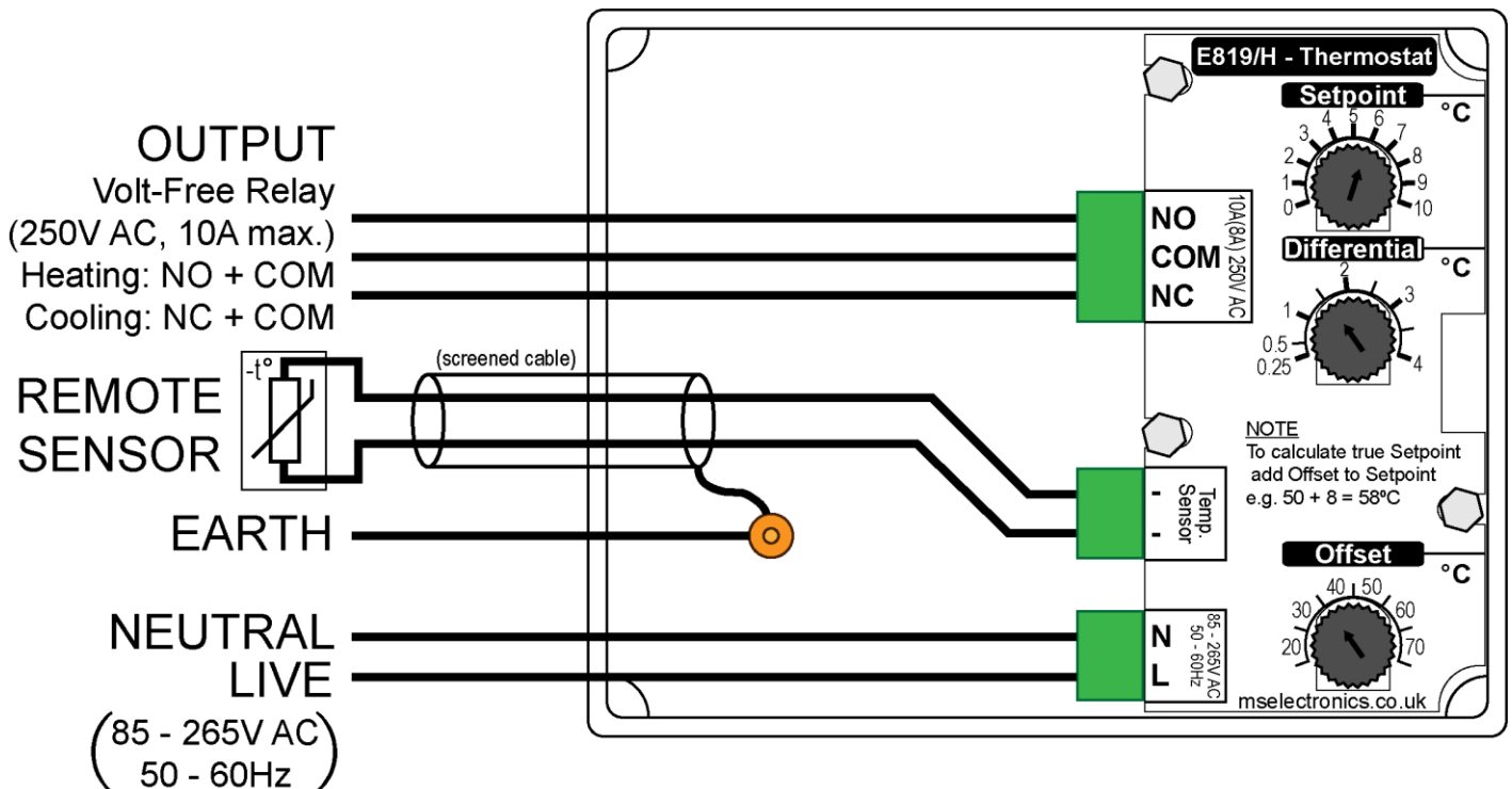
Figure 1 Typical wiring example (E819/H)
