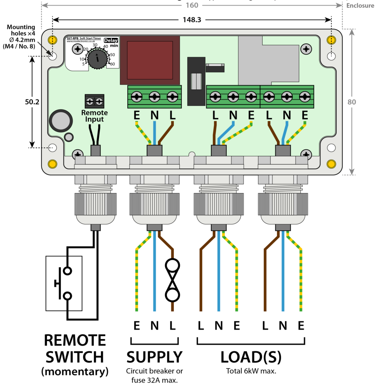
Figure 1 Typical wiring example and dimensions (in millimetres)
