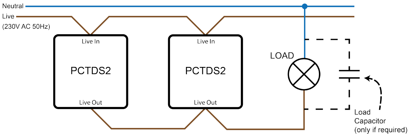
Figure 4 Typical ceiling rose plan
