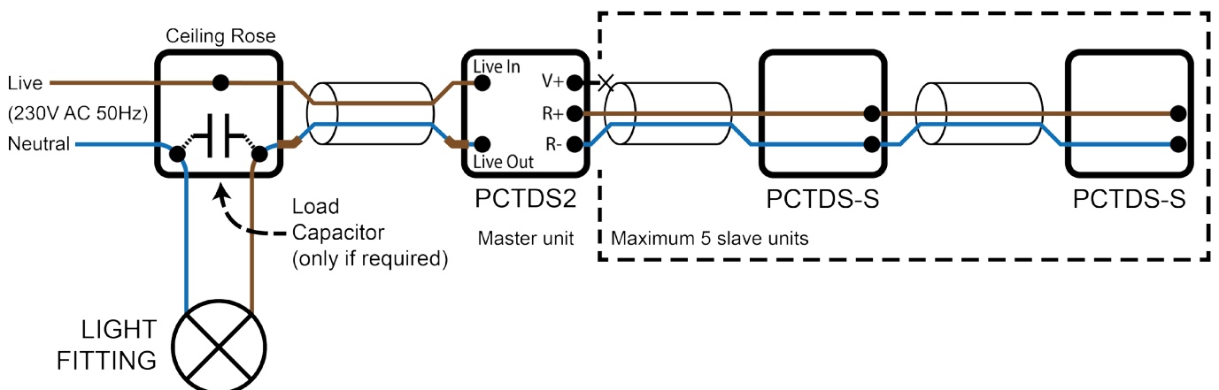
Figure 6 Typical ceiling rose plan using two PCTDS-S slave units
