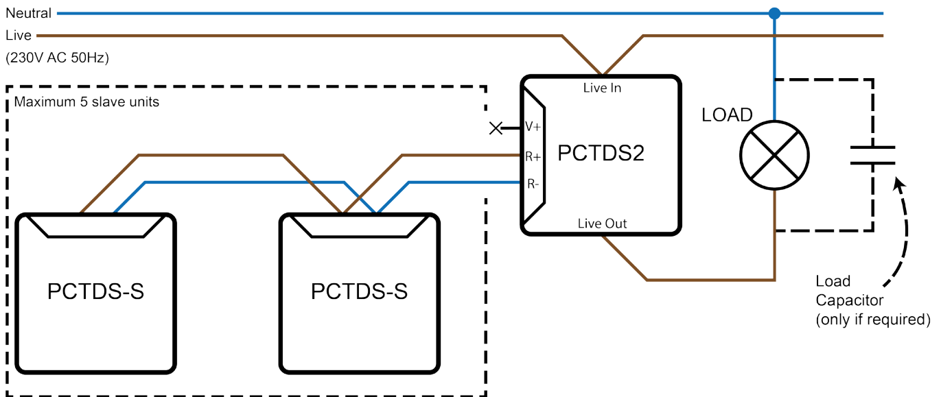
Figure 5 Typical wiring schematic using two PCTDS-S slave units
