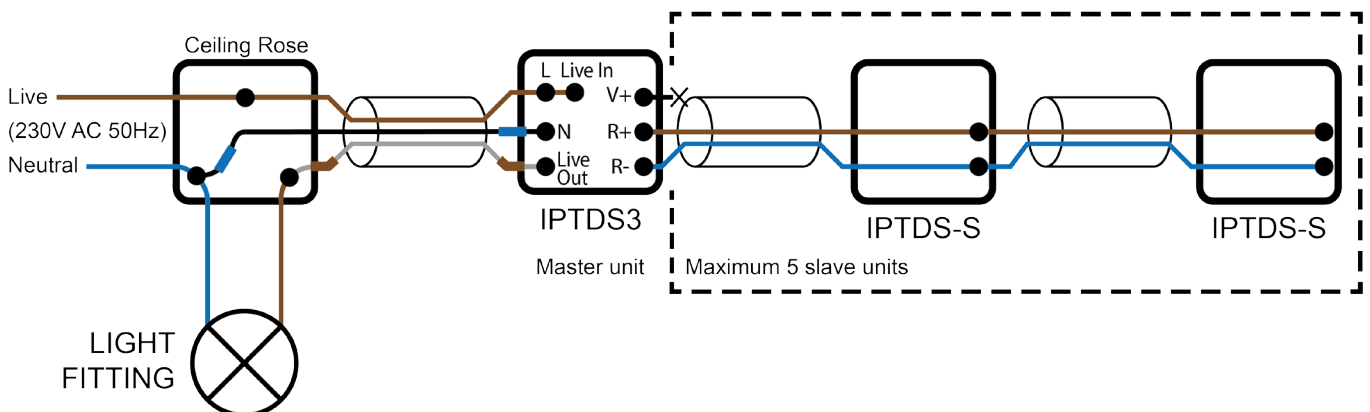
Figure 6 Typical ceiling rose plan using two IPTDS-S slave units
