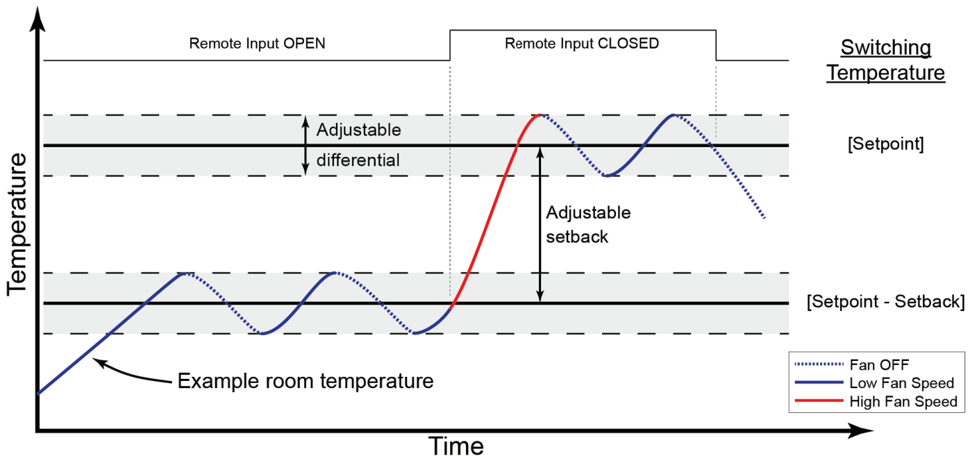
Figure 1 Functionality Diagram
