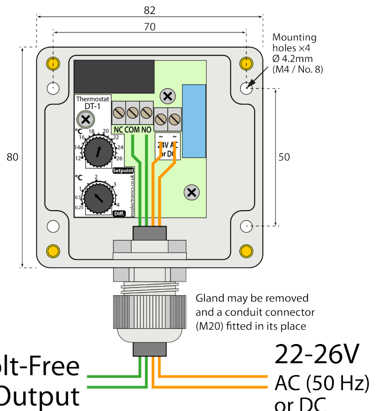
Figure 1 Typical wiring example (for heating)
