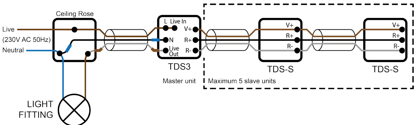
Figure 6 Typical ceiling rose plan using two TDS-S slave units
