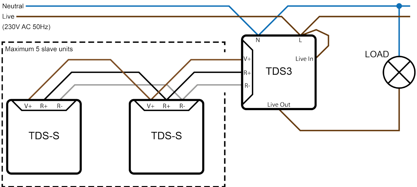
Figure 5 Typical wiring schematic using two TDS-S slave units
